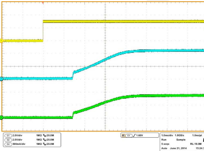
V_{IN}=5V, R_{OUT}=5.1\Omega, EN Startup
