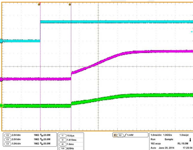
V_{IN}=5\text{V} , R_{OUT}=5\Omega , C_{OUT}=100\mu\text{F} , Turn on delay time
