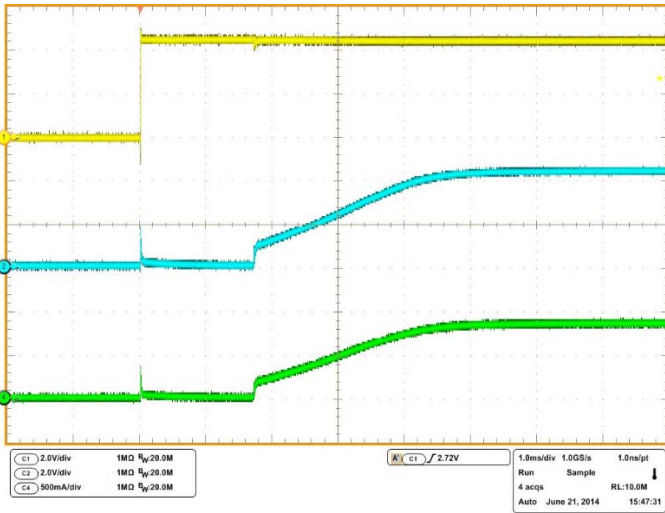
V_{IN}=5V, R_{OUT}=5.1\Omega, V_{IN} Startup
