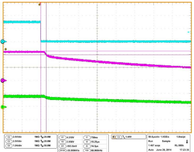
V_{IN}=5\text{V} , R_{OUT}=5\Omega , C_{OUT}=100\mu\text{F} , Turn off delay time
