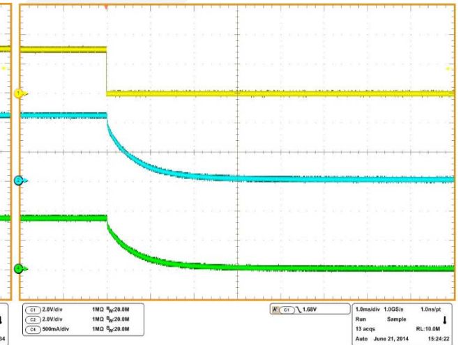
V_{IN}=5V, R_{OUT}=5.1\Omega, EN Shutdown
