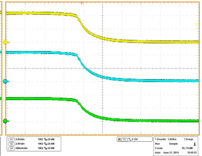
V_{IN}=5V, R_{OUT}=5.1\Omega, V_{IN} Shutdown
