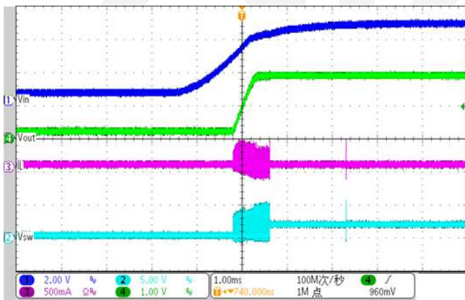
Vin Start up ( V_{in}=5V , V_{out}=1.8V , Load=0A)
