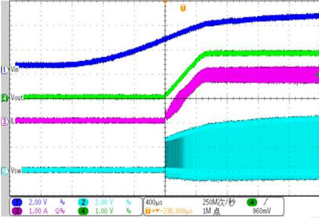
Enable Start up (Vin=5V, Vout=1.8V, Load=0A)
