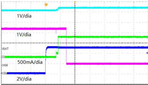
Figure 4. Power up
