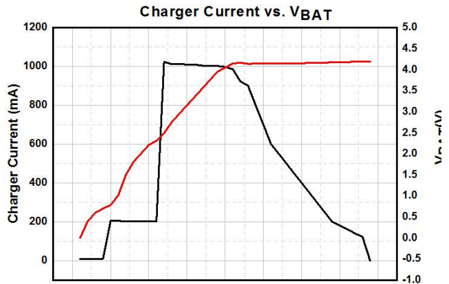
Figure 7. Charger Current vs. V BAT
