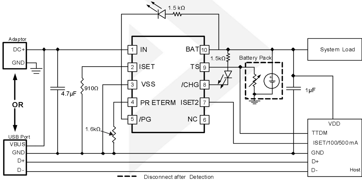
Figure 3. Typical Applications for DIO5840J
