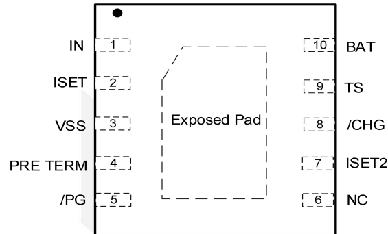
Figure 1. Top View
