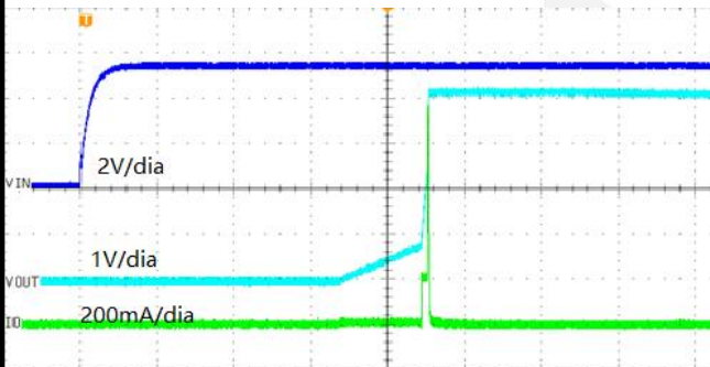
Figure 6. AC Charging
