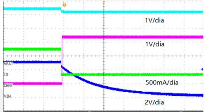
Figure 5. Power down
