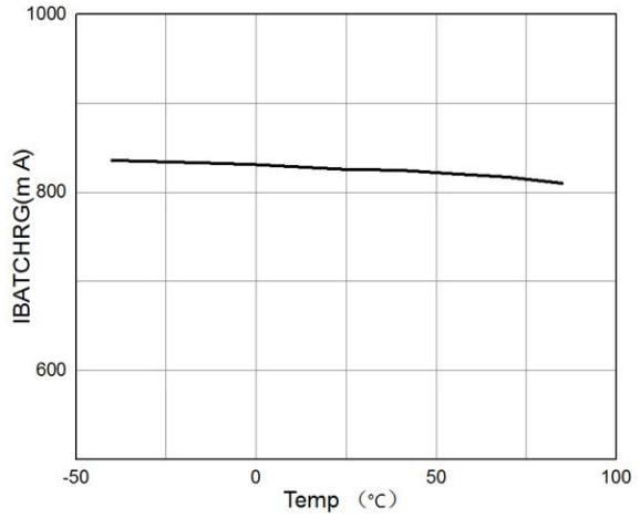
Figure 3. IBATCHRG vs Temp (VCC=5V, RISET=1K)
