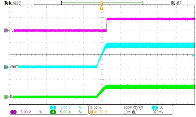
Figure 32. PG-OTP recovery
