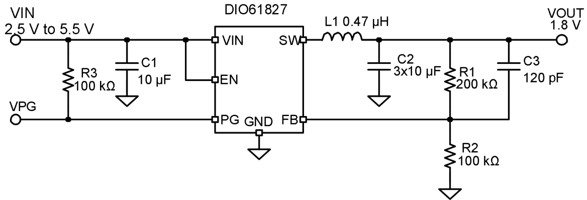
Figure 37. Typical applications
