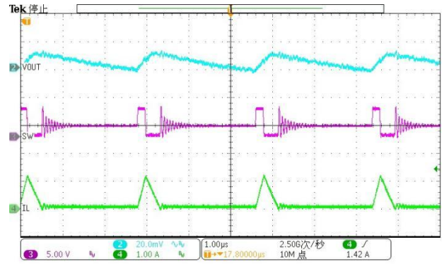
I_{OUT} = 0.1\text{ A} (DIO61825/6/7) Figure 14. PSM operation
