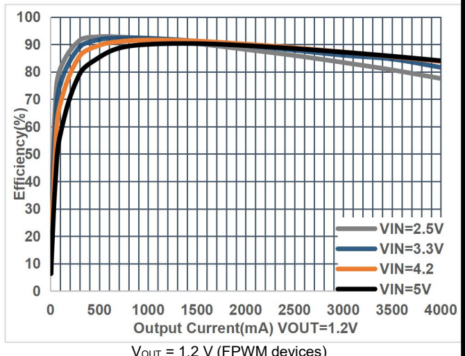
Figure 6. Efficiency
