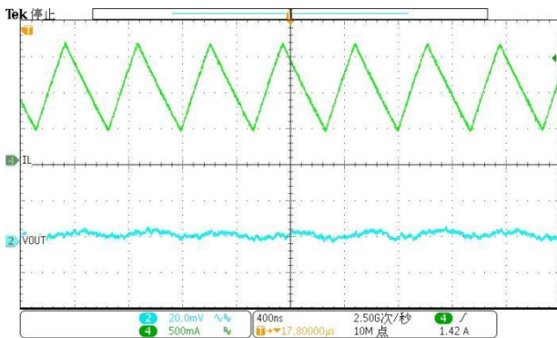
I_{OUT} = 1.0\text{ A} (DIO61825A/6A/7A) Figure 15. PWM operation at FPWM
