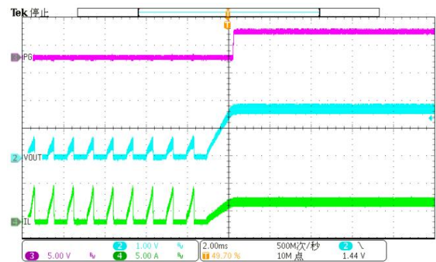
Figure 34. PG-SCP recovery
