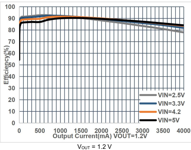
Figure 5. Efficiency
