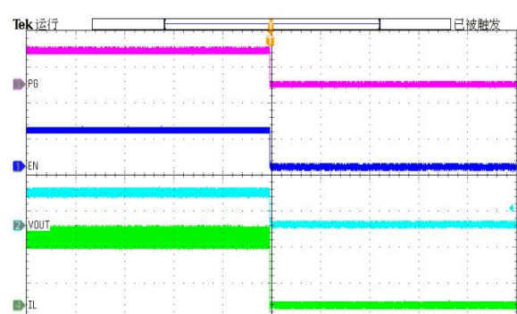
Figure 30. PG-discharge
