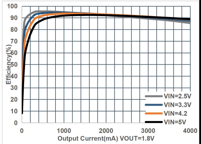
Figure 8. Efficiency
