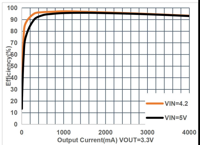
Figure 12. Efficiency
