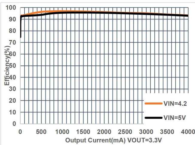
Figure 11. Efficiency
