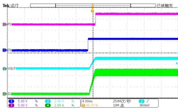
Figure 29. PG-start-up
