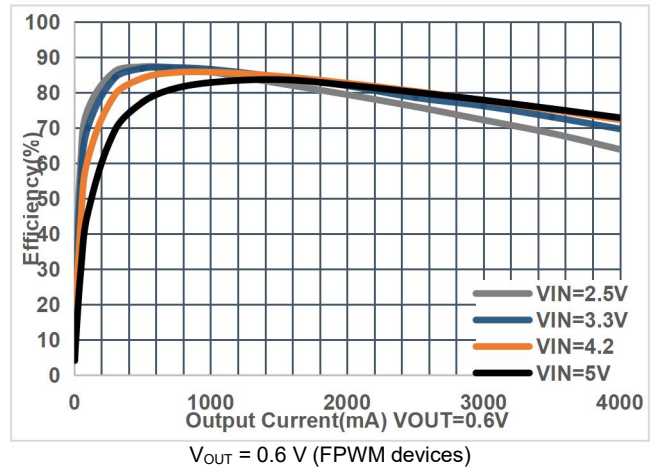
Figure 4. Efficiency
