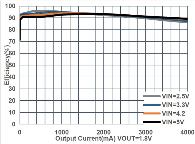
Figure 7. Efficiency
