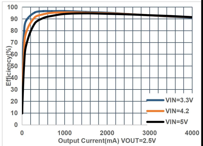
Figure 10. Efficiency
