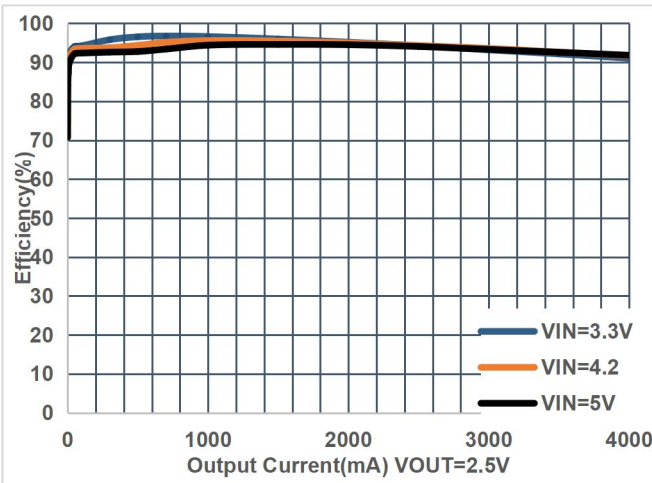
Figure 9. Efficiency
