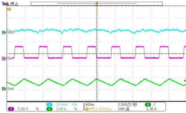
I_{OUT} = 1.0\text{ A} (DIO61825/6/7) Figure 13. PWM operation
