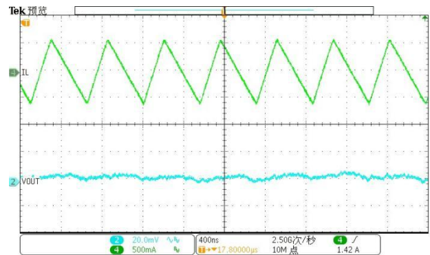
(DIO61825A/6A/7A) Figure 16. PWM operation at FPWM without load
