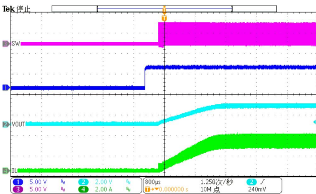
Load = 0.6\ \Omega (DIO61825/6/7) Figure 17. Start-up with load
