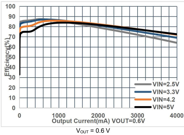
Figure 3. Efficiency
