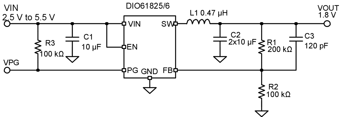
Figure 36. Typical applications
