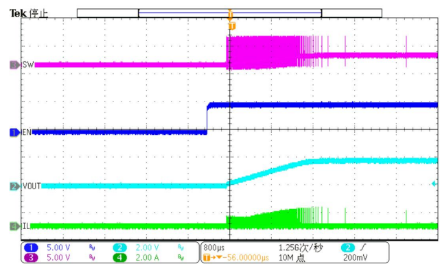
(DIO61825/6/7) Figure 18. Start-up without load
