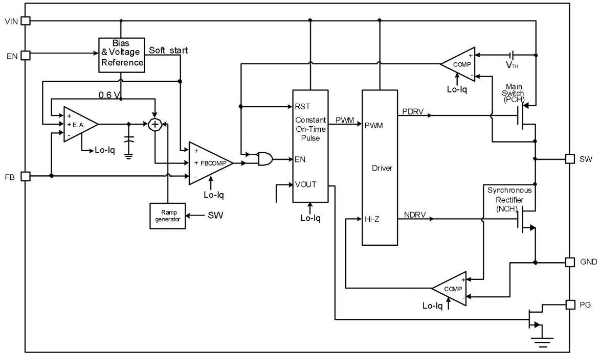
Figure 35. Block diagram
