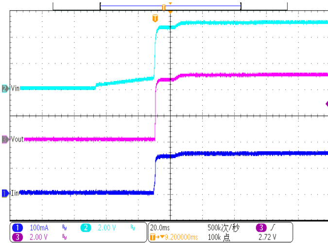
VIN Turn On (Vin=5V, Rload=33ohm)
