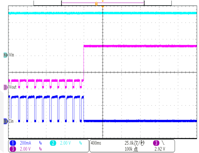
Over-Load to No-Load Transient Response (Vin=5V, Rload=2.7ohm)
