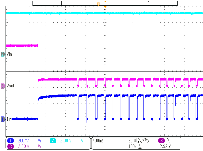
No-Load to Over-Load Transient Response (Vin=5V, Rload=2.7ohm)
