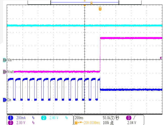
Short-Circuit to No-Load Transient Response (Vin=5V)
