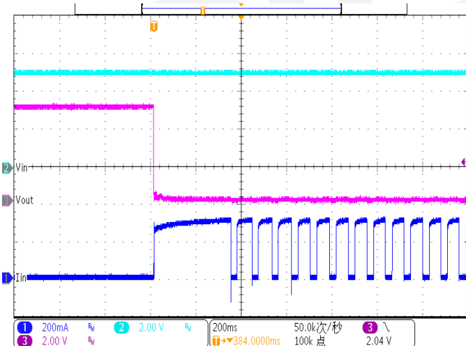
No-Load to Short-Circuit Transient Response (Vin=5V)
