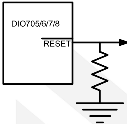
Figure 6 RESET Valid to Ground Circuit
