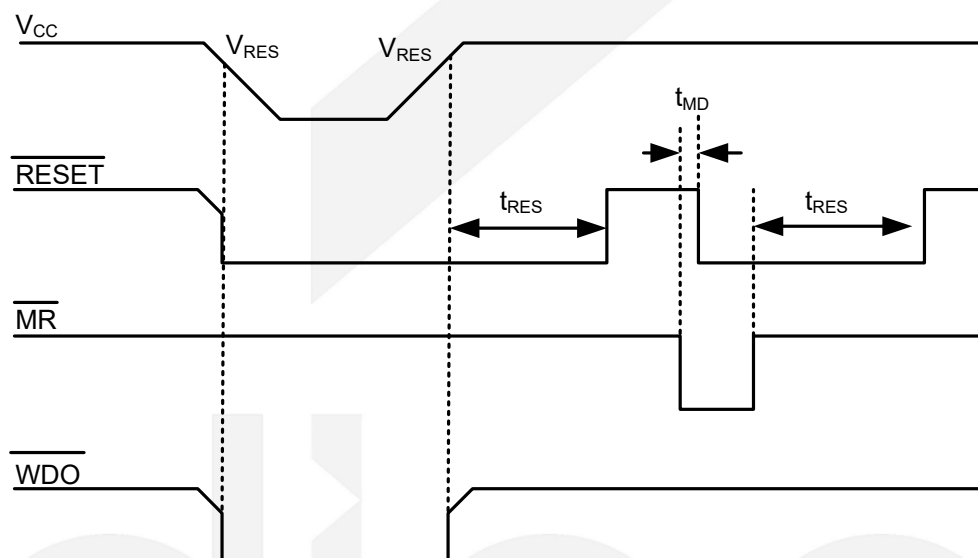
Figure 4. Watchdog Timing
