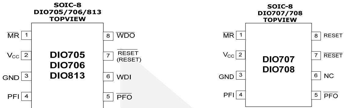
Figure 1 Pin Assignment
