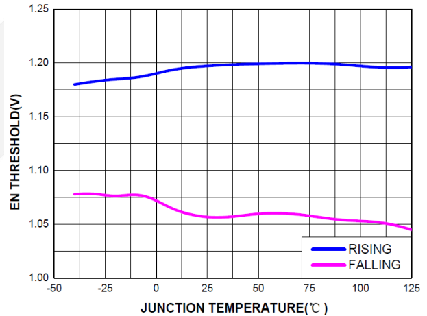
Figure 6. EN Threshold vs. Junction Temperature
