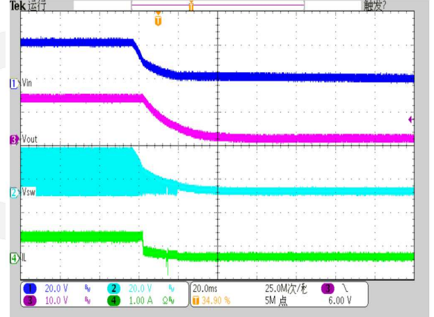
I_{out} = 0.6A
