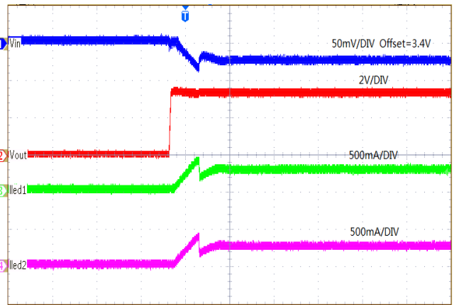
Time (1ms/DIV)
