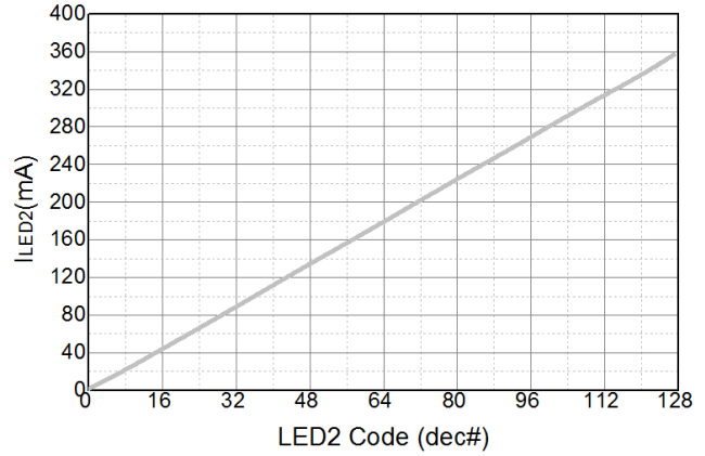
LED2 Torch Current x2 vs. Brightness Code
