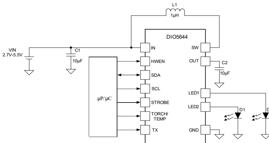
Figure 4. Application Circuit
