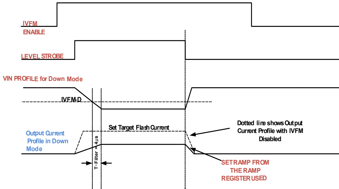
Figure 6. Down Mode
