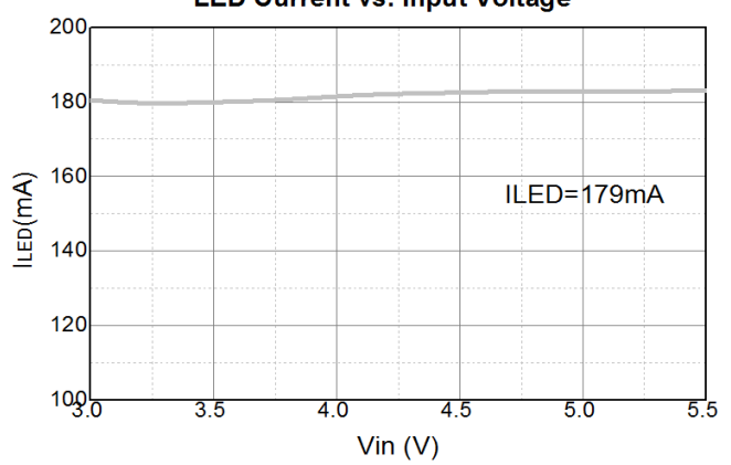
Figure 24. Torch Mode LED Current vs Input Voltage
