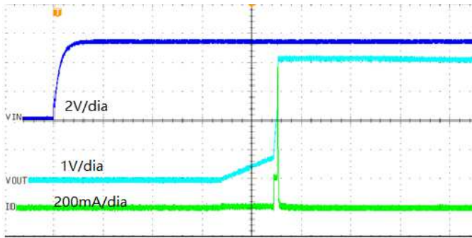
Figure 6. AC Charging
